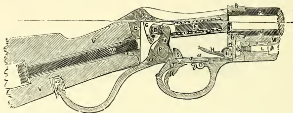
The Martini-Henry Breech-loader and its Parts.
